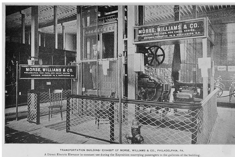
Figure 11: Photographic view of Morse, Williams & Company's exhibit, a working electric elevator, at the World's Columbian Exposition in Chicago in 1893.
