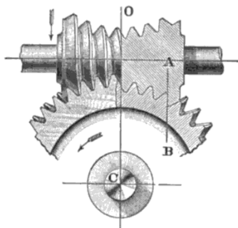
Figure 7 (left): Illustration of the Hindley Screw, which Morse, Williams & Company were the first to implement in elevator machinery. The company held the exclusive right to this innovative type of gearing for many years, making their elevators some of the most efficient on the market.
