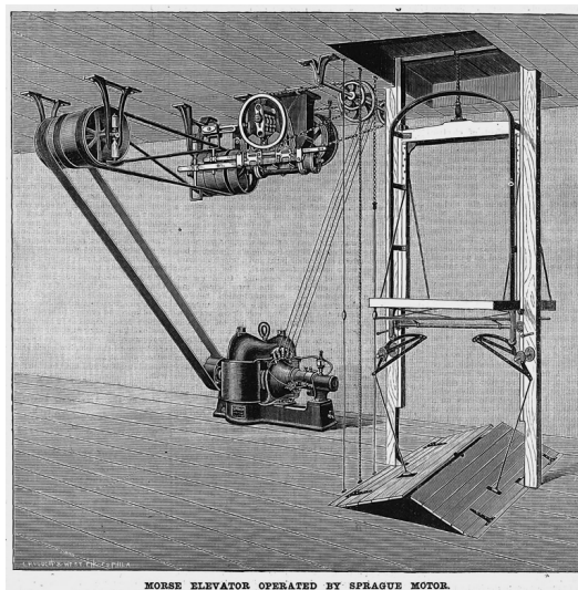
Figure 10: Illustration of a Morse elevator equipped with the Sprague electric motor.
