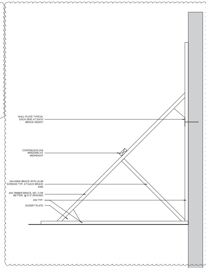
4 NEW WALL INFILL & SHORING DETAILS 1 1/2" = 1'-0"
