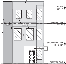
7 REAR ELEVATION 1/8" = 1'-0"
