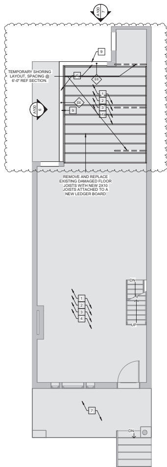
1 FIRST FLOOR - ARCH 1/4" = 1'-0"
