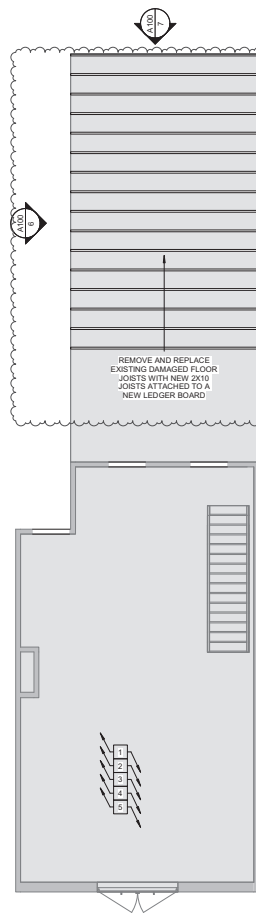
3 THIRD FLOOR - ARCH 1/4" = 1'-0"
