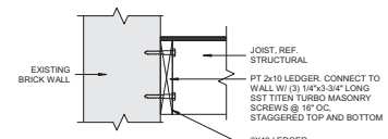
9 LEDGER DETAIL 1 1/2" = 1'-0"
