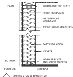
WALL TYPES
