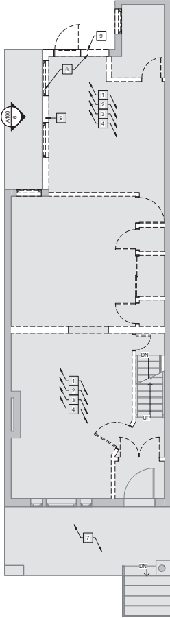
2 FIRST FLOOR - DEMO 1/4" = 1'-0"
