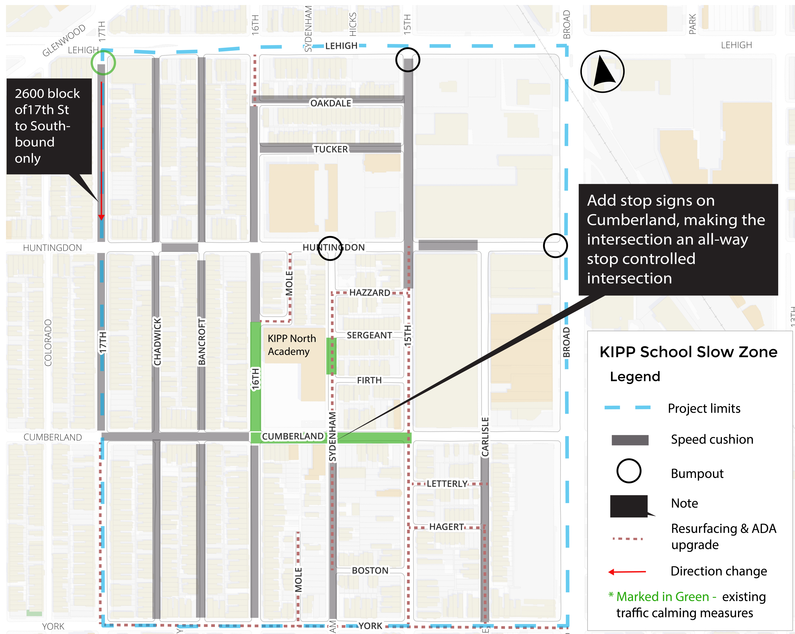
Speed cushions Topes segmentados
