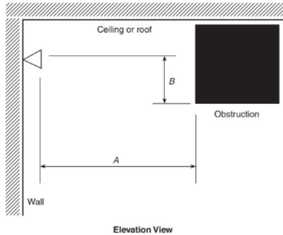
FIGURE 10.3.6.1.3 Positioning of Sprinkler to Avoid Obstruction (Standard Sidewall Spray Sprinklers).
