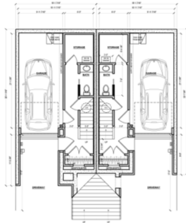
BASEMENT PLAN
