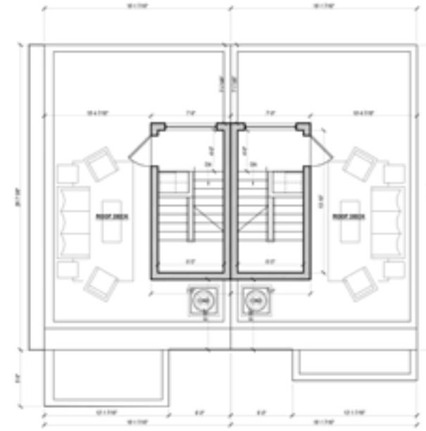
ROOF PLAN
