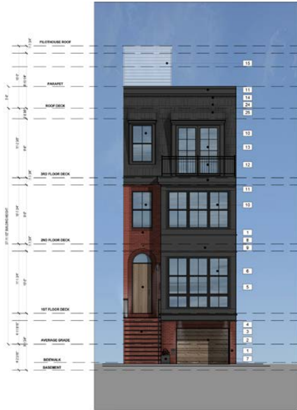
1 - FRONT ELEVATION
