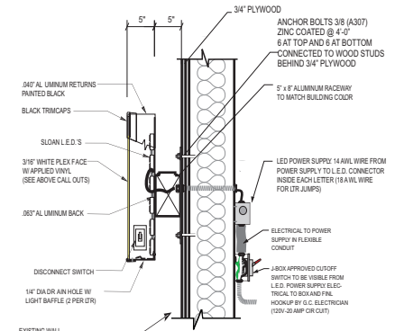
SIGN MOUNTING DETAIL scale 1/2"=1'
