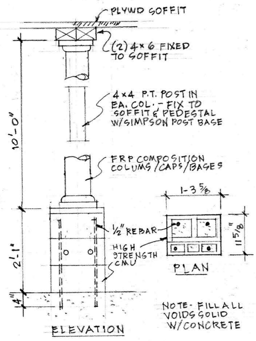
COLUMN & PEDESTAL DETAILS 3/4" = 1'-0"
