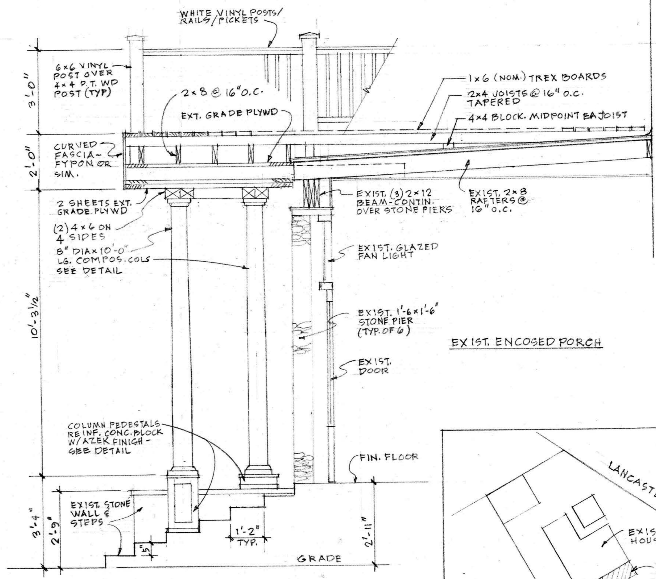
SECTION A-A 1/2" = 1'-0"
