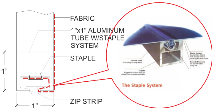
D2 TYP. SECTION STAPLED Scale: NTS
