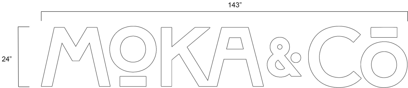
QTY 1: LED ILLUMINATED FRONT-LIT CHANNEL LETTERS
