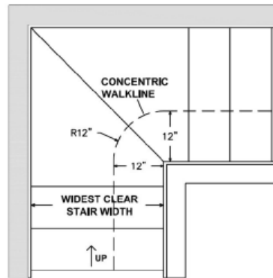
FIGURE R311.7.4 WINDER TREAD AND LANDING DETAIL
