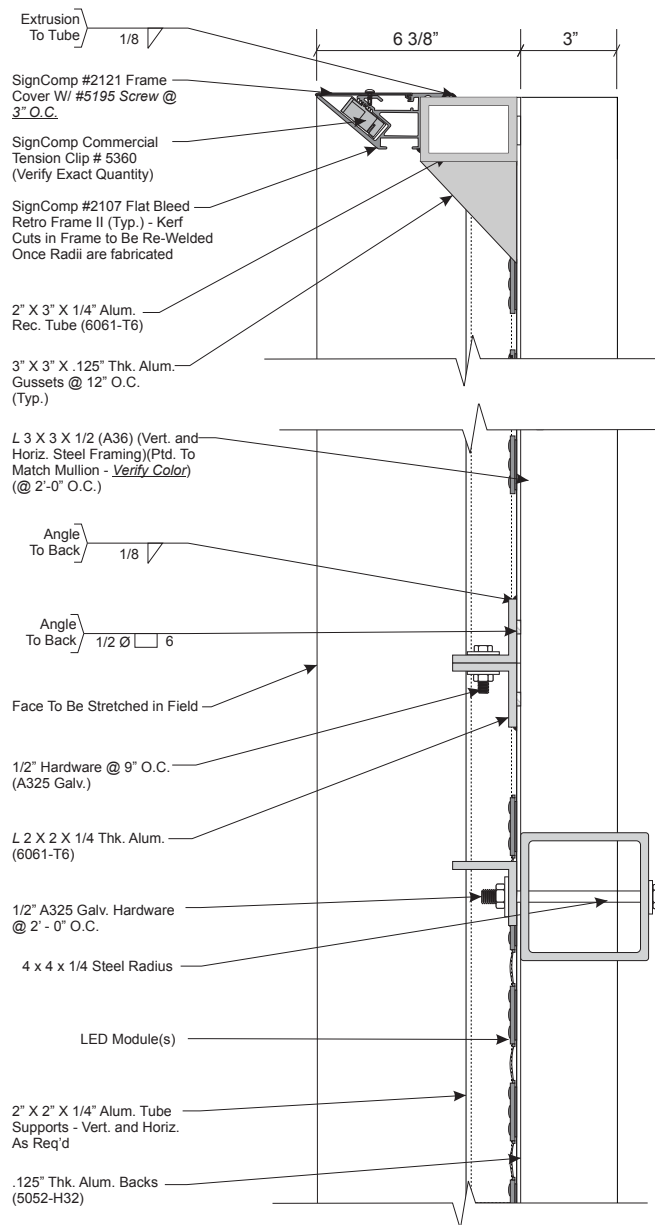
TYPICAL CHANNEL LETTER SECTION
