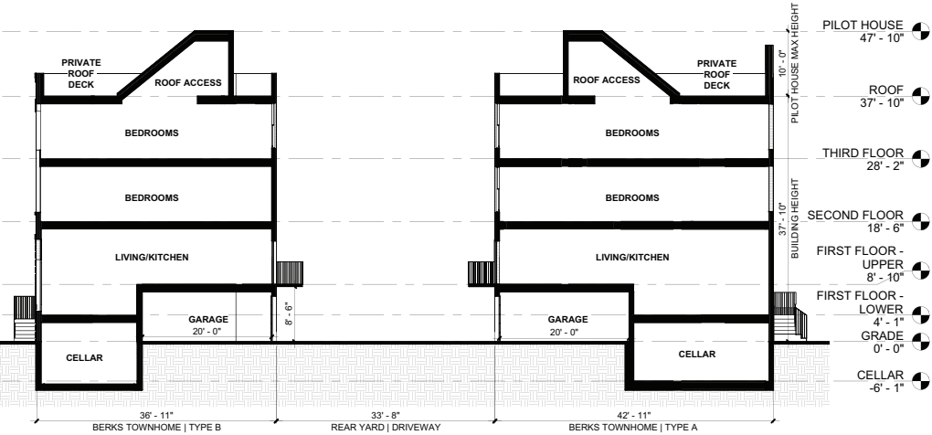
2 Z-1 ZONING SECTION - TOWNHOME TYPES A & B 3/32" = 1'-0"
