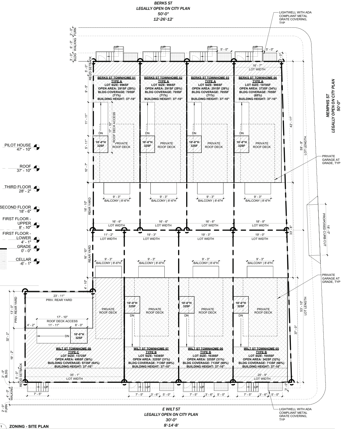
1 Z-1 ZONING - SITE PLAN 1/8" = 1'-0"
