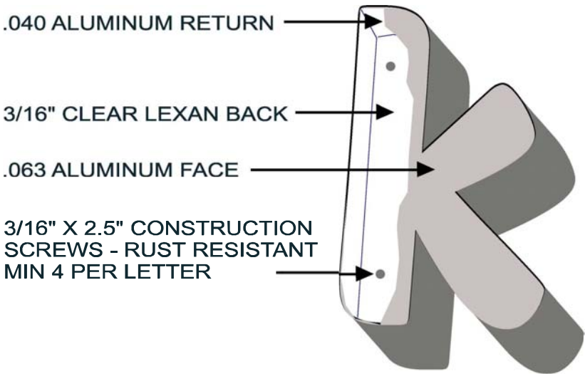
Fabricated Metal Letter FRONT VIEW
