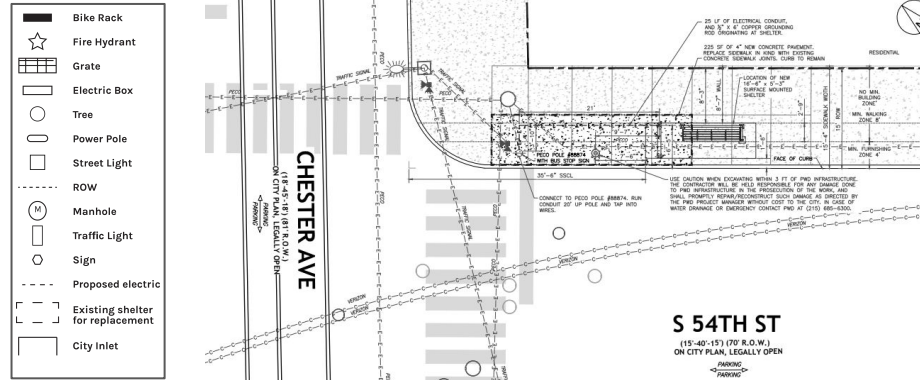
SITE PLAN
