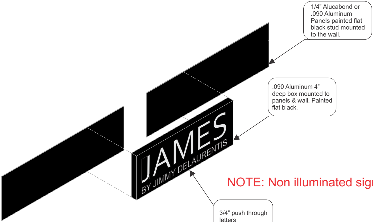
D Exploded SW Isometric 1.0 NOT TO SCALE
