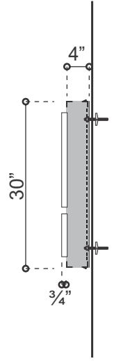
B Side Section View 2.0 Scale= 1/2" = 1'-0"
