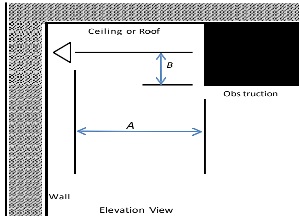
FIGURE 6.4.6.3.7.2(a) Positioning of Sprinklers to Avoid Obstructions (Residential Sidewall Sprinklers)
