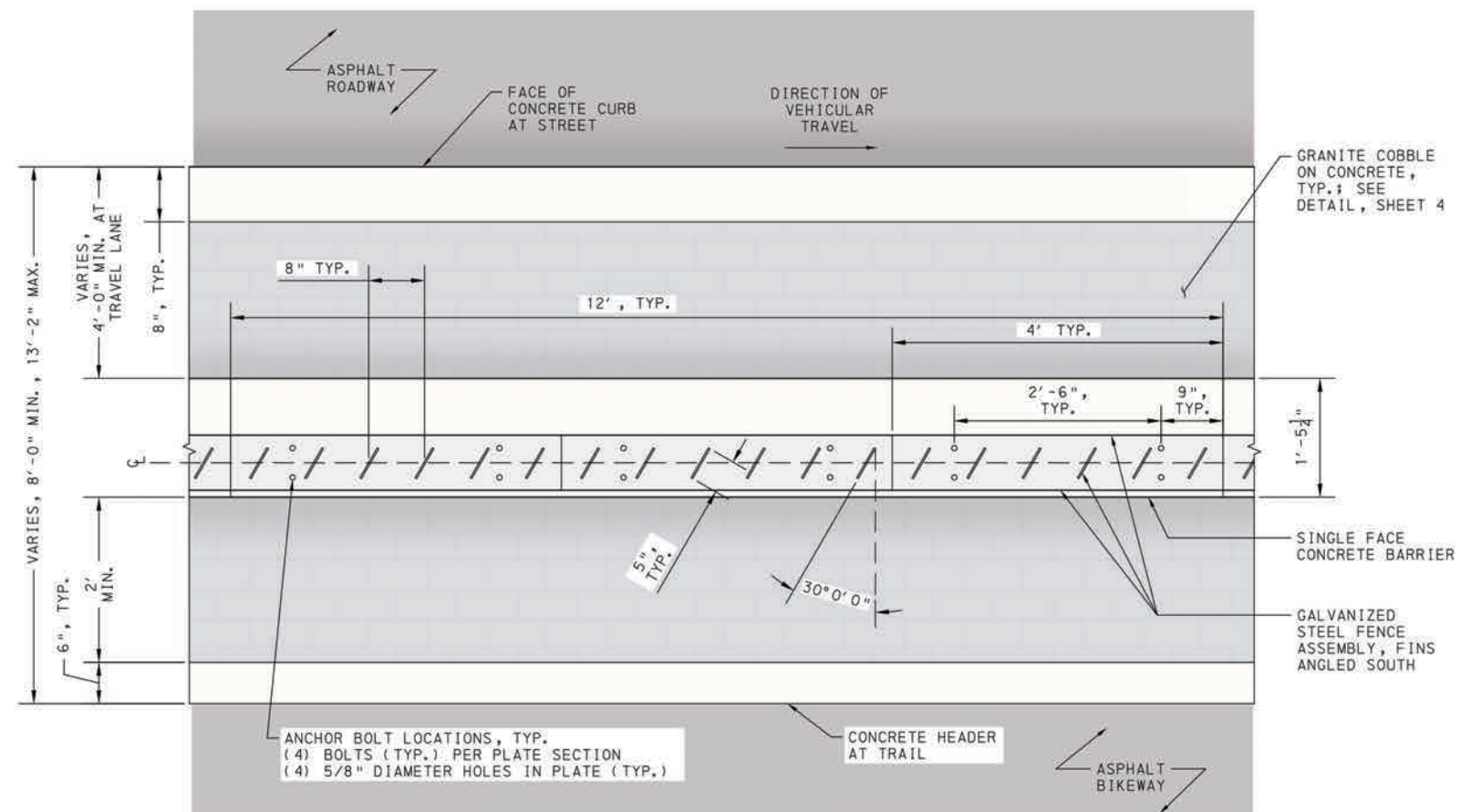
TRAIL BUFFER FENCE AND BARRIER PLAN (ITEM 9000-2155)
