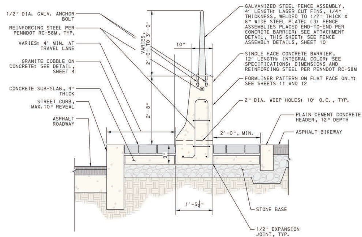
TRAIL BUFFER FENCE AND BARRIER SECTION (ITEM 9000-2155)
