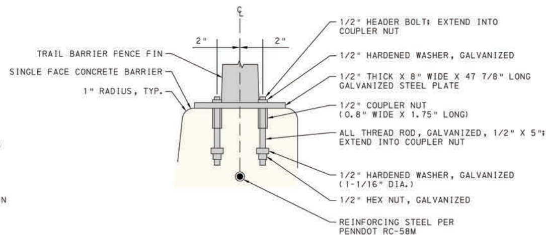
FENCE ASSEMBLY ATTACHMENT TO CONCRETE BARRIER (ITEM 9000-2155)
