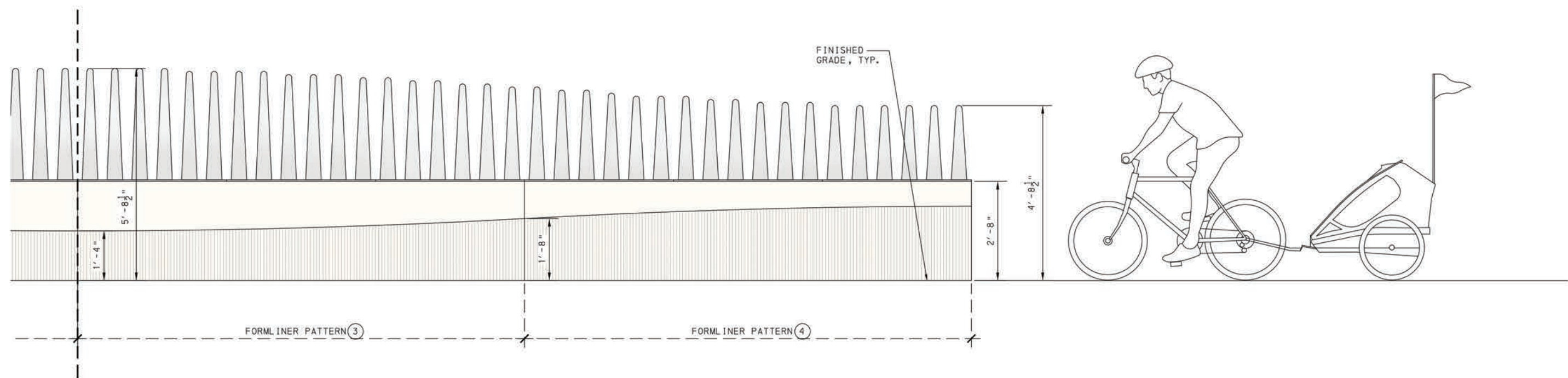
TRAIL BUFFER BARRIER CONCRETE FORMLINER PATTERNS (ITEM 9000-2155)
