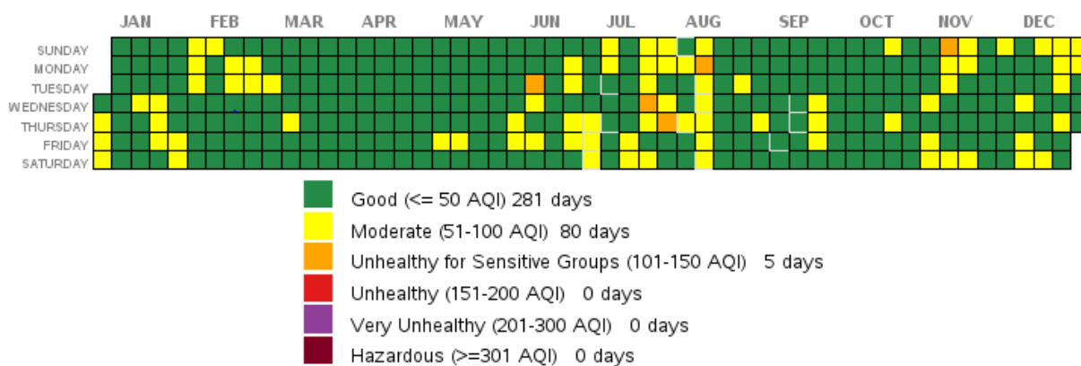
Figure 3.1 – Daily AQI Values for 2020
