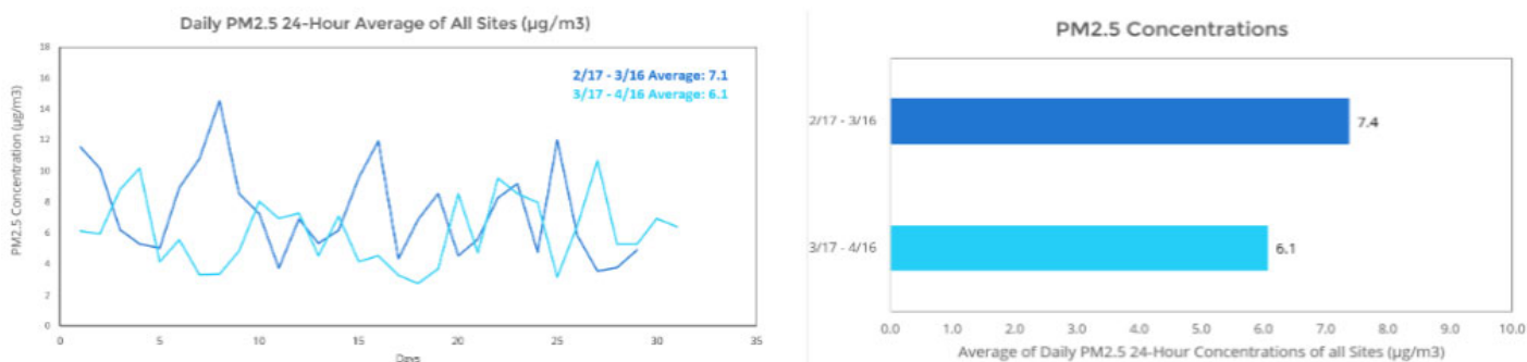
Figure 13.2 – Daily 24-Hour PM 2.5 (µg/m 3 ) One Month After Shutdown vs. One Month Before Shutdown
