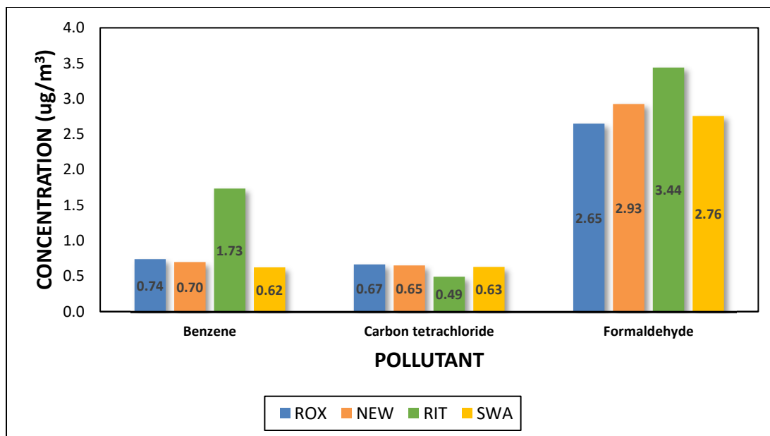
Figure 11.4 – 2020 Mean Concentrations for Benzene, Carbon Tetrachloride, and Formaldehyde 9
