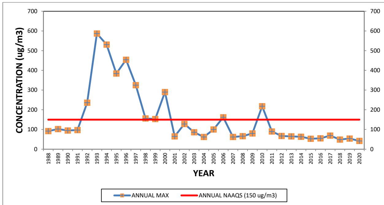
Figure 9.2 – PM 10 Trends for the Highest 24-Hour Average Concentration for All Monitoring Sites
