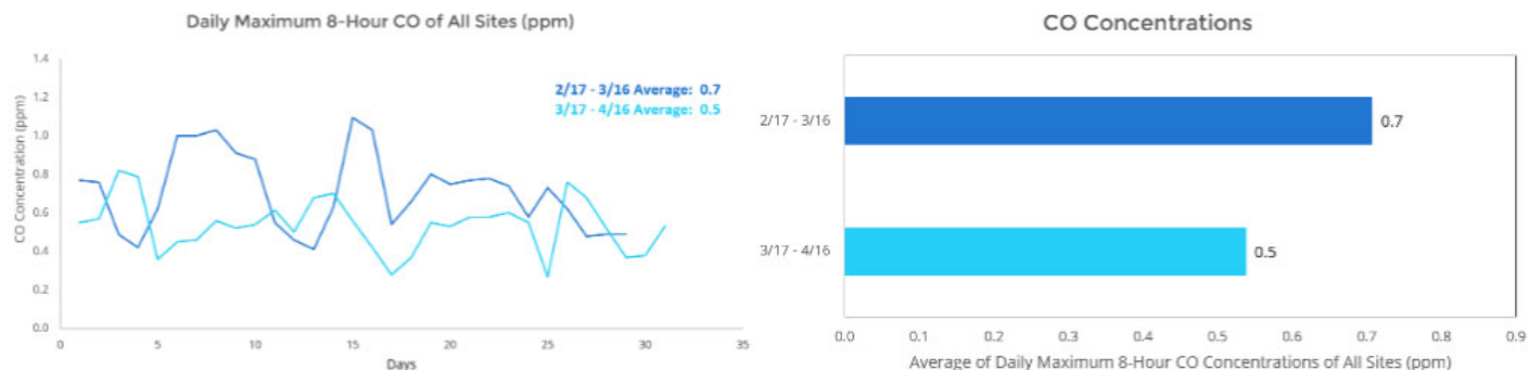
Figure 13.3 – Daily Maximum 8-Hour CO (ppm) One Month After Shutdown vs. One Month Before Shutdown
