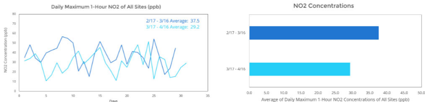
Figure 13.1 – Daily Maximum 1-Hour NO 2 (ppb) One Month After Shutdown vs. One Month Before Shutdown
