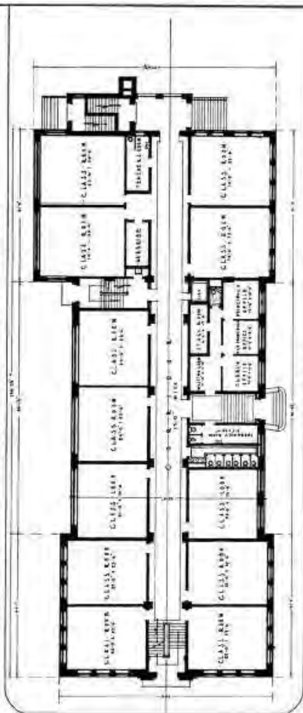
-PLAN OF FIRST FLOOR-
