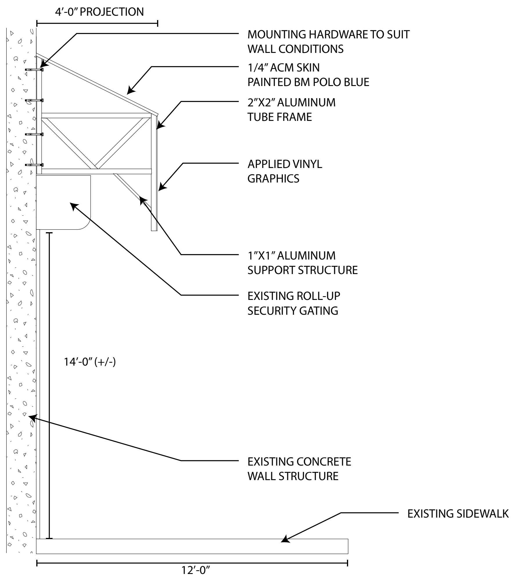
A AWNING DETAIL PROJECTED VIEW OF AWNING OVER EXISTING SIDEWALK
