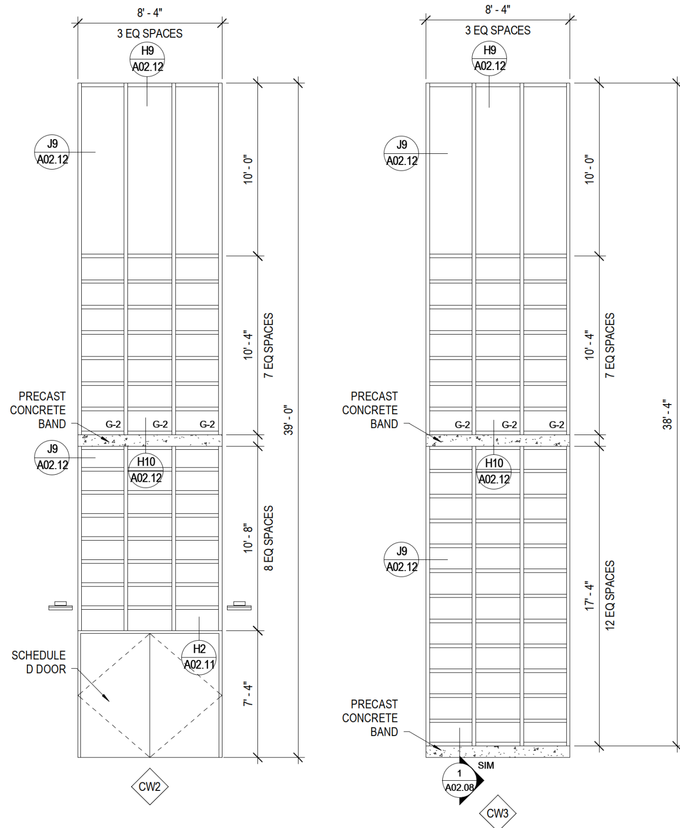
CURTAIN WALL SCHEDULE
