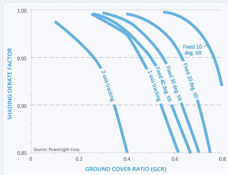
Figure 3-5: Shading derate factor for multiple-row PV arrays as a function of PV array type and ground cover ratio
